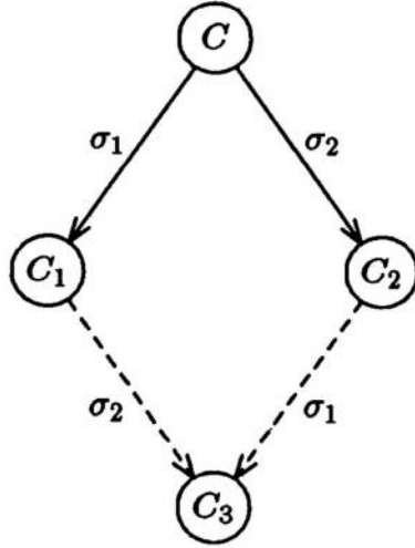
Figure 12.1: Two schedules that do not involve a common node are commutative — see Lemma 13.
